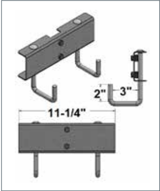
1/2" CARRIAGE BOLT ADJUSTABLE HOOK • ZINC FINISH
